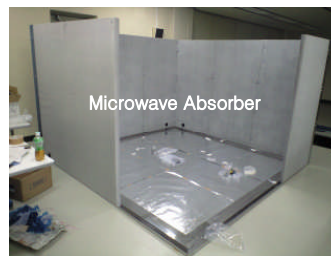
Light Anechoic Chamber for Mobile R&D 2.4m×2.4m
