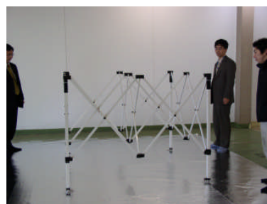
Al. Frame
