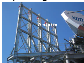
Reflection Reduction at 6.3GHz Antenna
